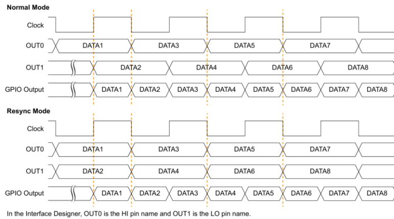
Figure 17: DDIO Output Timing Waveform
