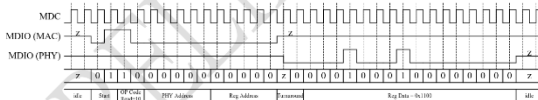
Figure 1 MDC/MDIO Read Timing
