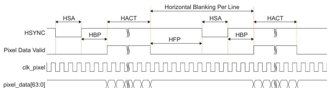
Figure 2: Video Timing Waveform (Horizontal)
