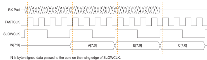
Figure 29: LVDS RX Timing Example Serialization Width of 8 (Half Rate)
