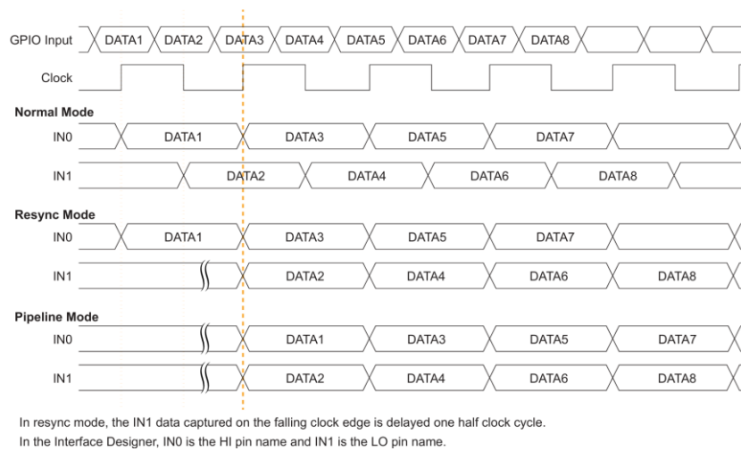
Figure 16: DDIO Input Timing Waveform
