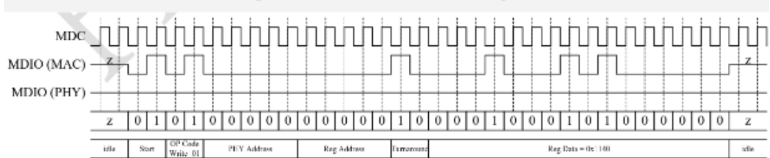
Figure 2 MDC/MDIO Write Timing
