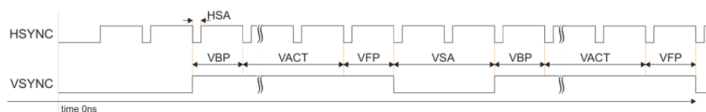
Figure 3: Video Timing Waveform (Vertical)
